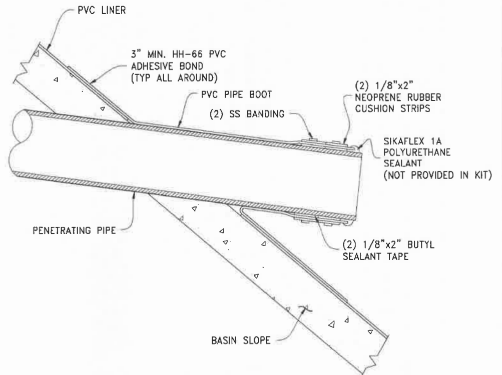
SLOPED PVC PIPE PENETRATION BOOT DETAIL
