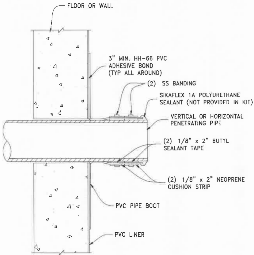
STRAIGHT PVC PIPE PIPE PENETRATION DETAIL
